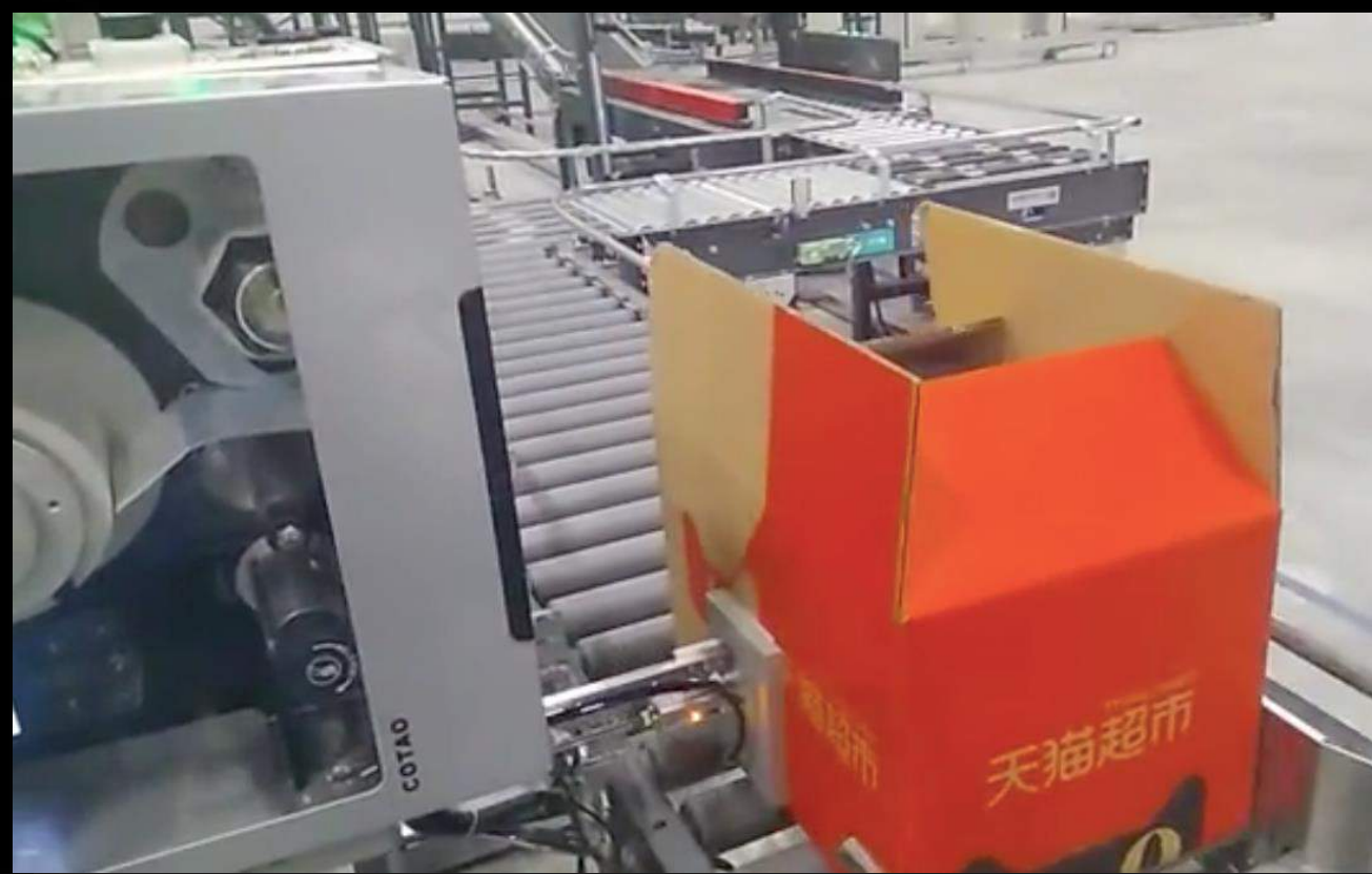
➤ Auto-labeling machine
